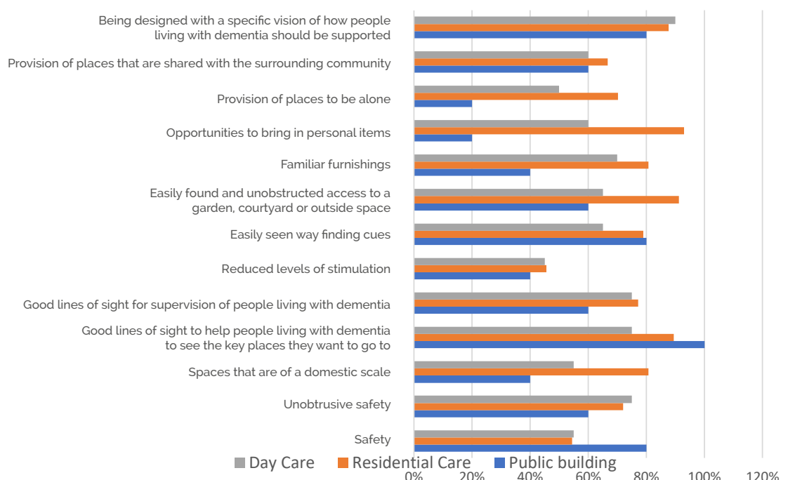
Figure 4. Relative importance of examples of design principles
