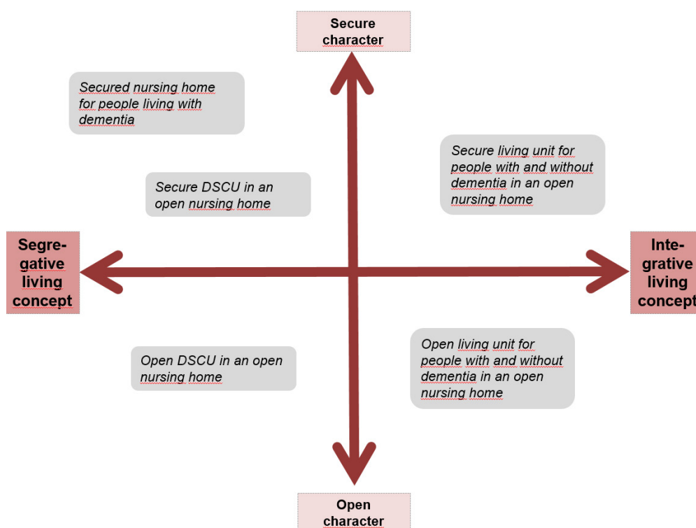
Figure 1: Possibilities for integrative and segregative living concepts (DSCU = Dementia Special Care Units)
